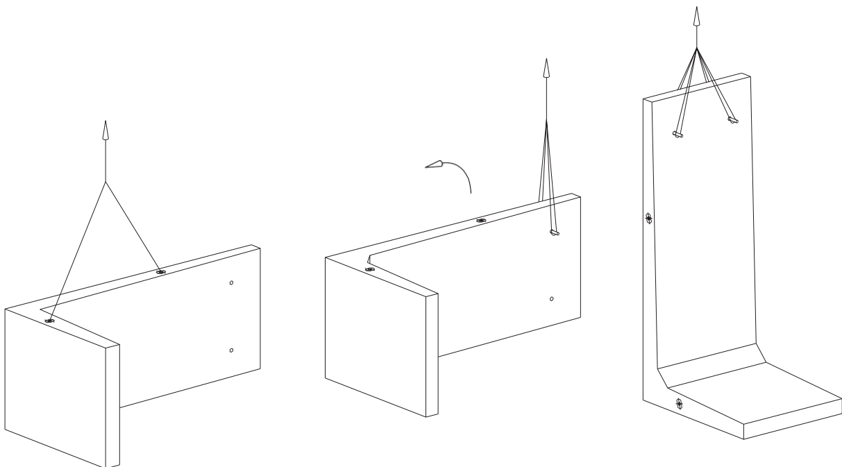
De-Mould and Transportation Diagram (nts)
