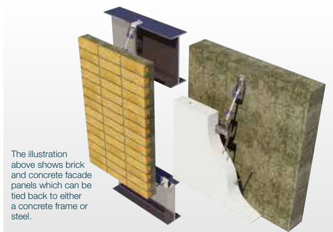
Facade panels
