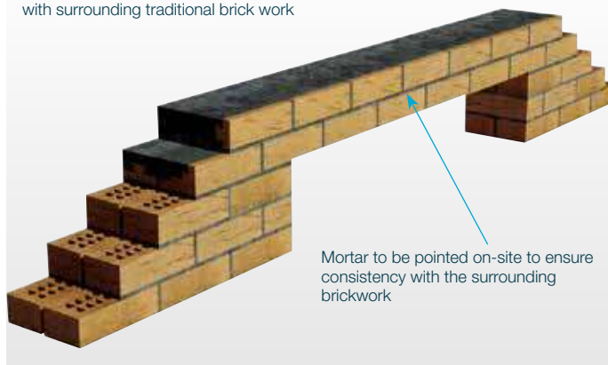
Bearing Lintels
