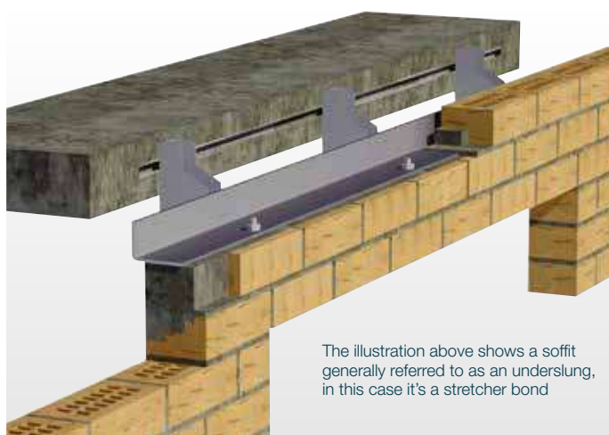
Underslung brick-faced soffits
