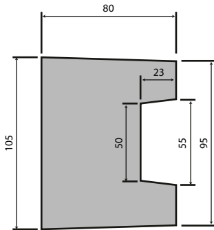
End Post
