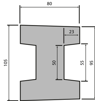
Intermediate Post
